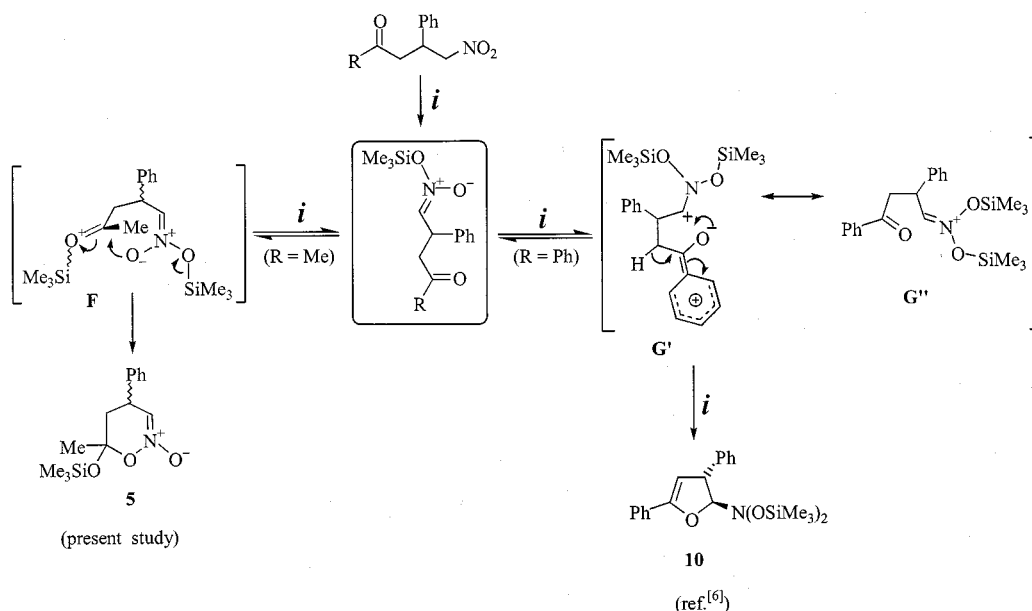
Scheme 3. i. \text{Me}_3\text{SiBr}/\text{Et}_3\text{N} in \text{CH}_2\text{Cl}_2 , -30^\circ\text{C}
